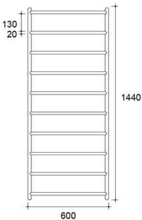
Front Elevation
