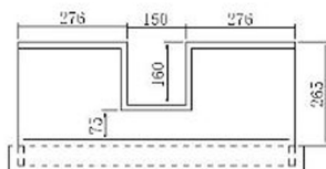
Planfrom View for drawer
