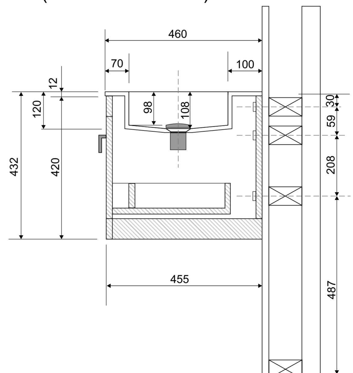
BASIN & CABINET: SECTION (SIDE ELEVATION)
