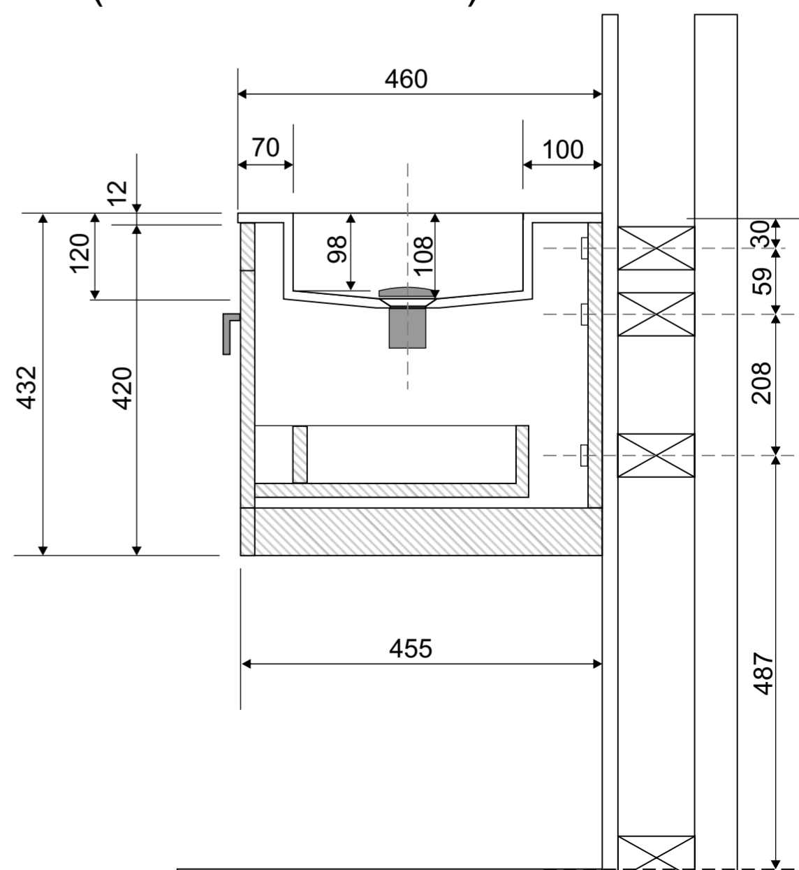
BASIN & CABINET: SECTION (SIDE ELEVATION)
