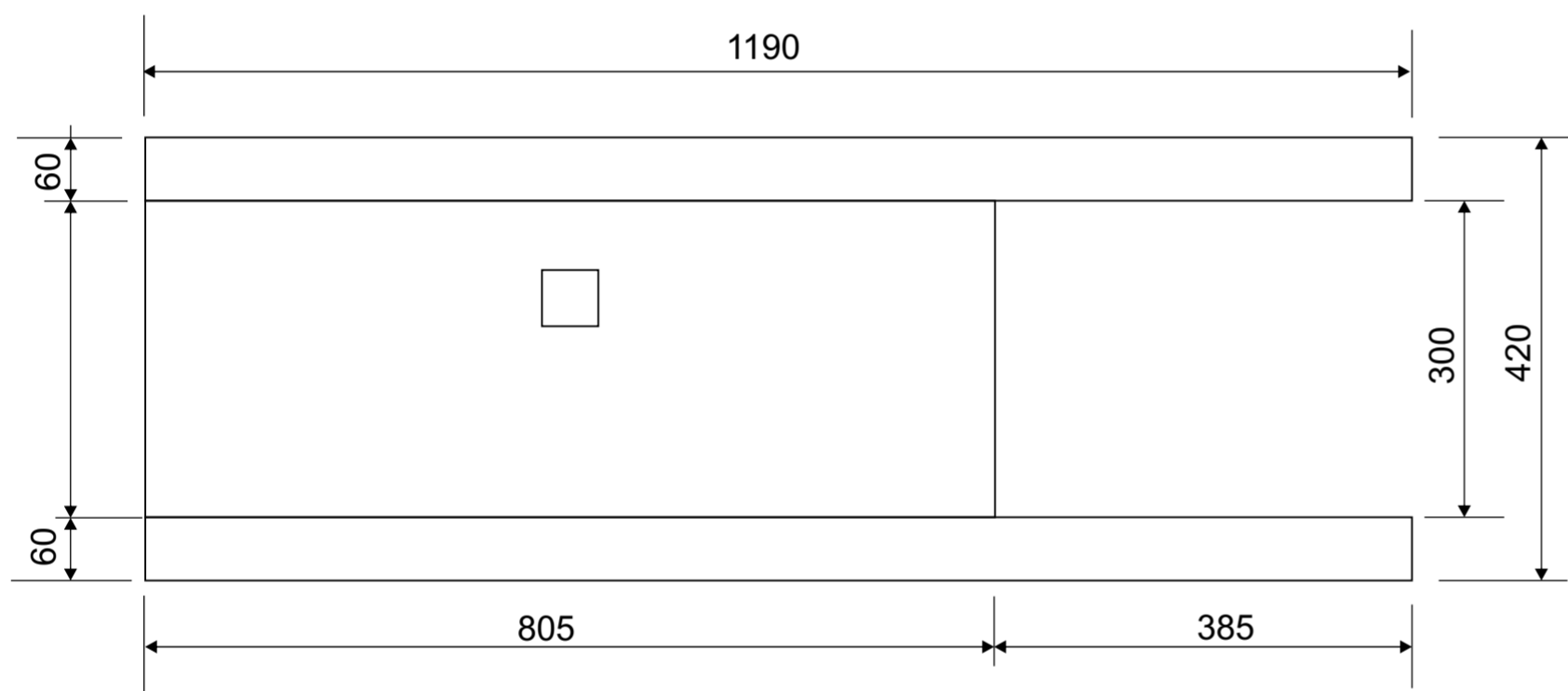
CABINET: FRONT ELEVATION
