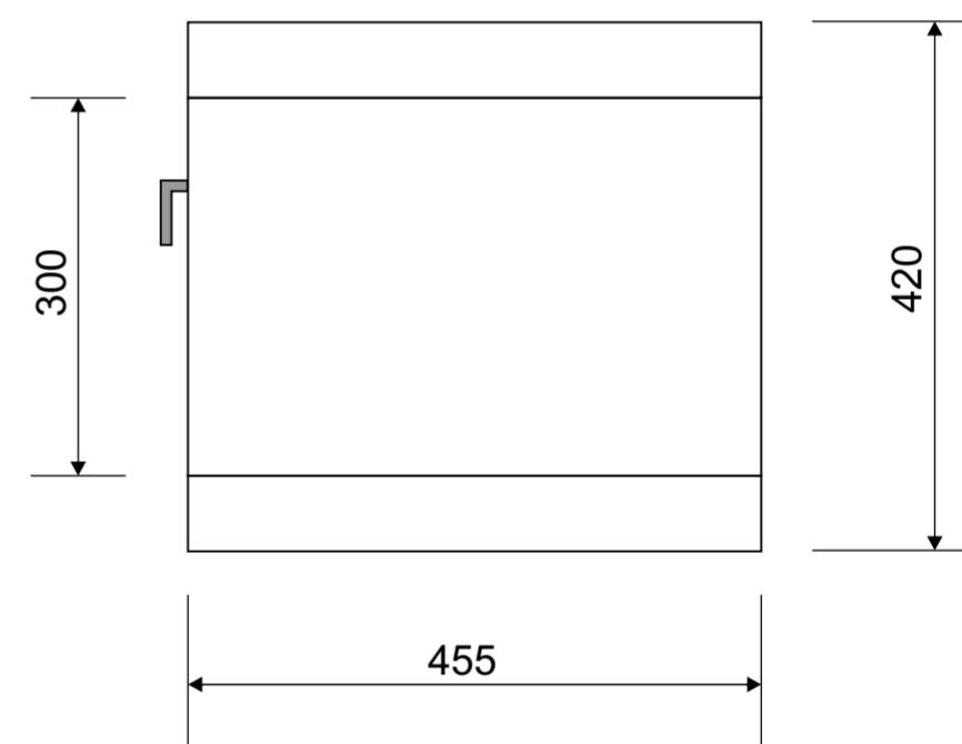
CABINET: SIDE ELEVATION
