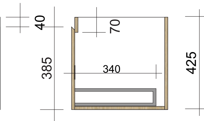
Side Section
